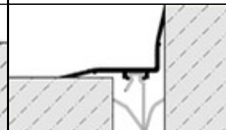
Corner profile
