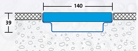
DW-DRAIN DWD 140
