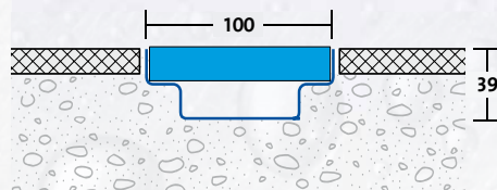
DW-DRAIN DWD 100
